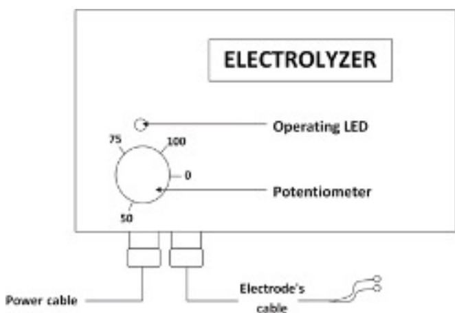
Front view of the electrolyzer
